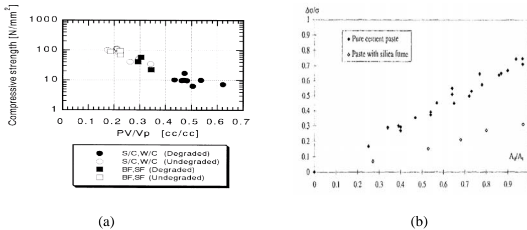
Figure 9 – (a) Relationship between porosity ( \text{PV}/\text{Vp} ) and compressive strength for sound and degraded materials [Saito00] and (b) variation of the strength loss in relation to the degradation ratio A_d/A_t [Carde96].
