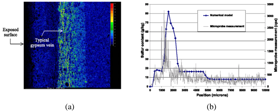
Figure 16 – Sulfur content mapping (a) and sulfur profiles (b) for 0.6 W/C ratio CSA Type 10 cement pastes exposed for 3 months to a 50 mmol/l \text{Na}_2\text{SO}_4 solution [Maltais04].
