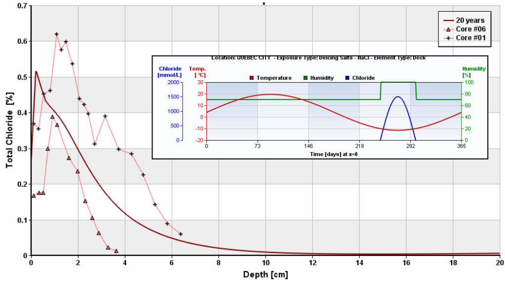
Figure 2 – Predicted total chloride profile in a 20-year-old parking structure using the model presented in [Samson07], compared to measurements performed on two cores. The inserted graph illustrates the time-dependent boundary conditions over one year.
