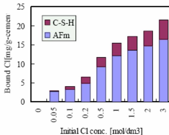
Figure 1 – Contribution of the chloride chemical binding with AFm and physical binding with C-S-H in a cement system (from ref. [Hosokawa06])
