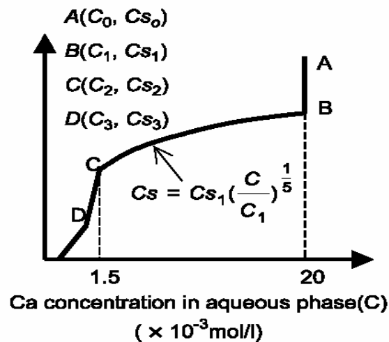
Figure10 – Relationship between Ca concentrations in the solution and the solid from Daimon et al. [Haga05, Daimon77]
