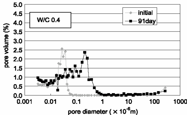
Figure 7 – Pore size distribution of the initial sample and that leached for 91 days [Haga05].
