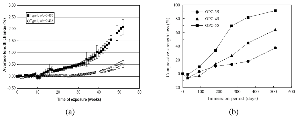
Figure 12 – Expansions of mortars under sodium sulfate attack as a function of W/C : (a) [Naik2006] and (b) [Lee05]
