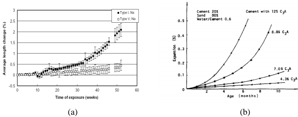
Figure 13 – Expansions of mortars under sodium sulfate attack as a function of C_3A content : (a) \%C_3A_{typeI} > \%C_3A_{typeV} [Naik2006] and (b) [Ouyang1988]
