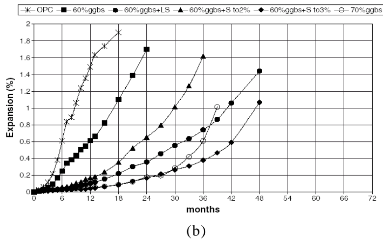
Figure 14 – Expansions of Sandberg prisms for different slag content: (a) in Na 2 SO 4 solution (1.5 % SO 3 ) and (b) in MgSO 4 solution (1.5 % SO 3 ) [Higgins03]
