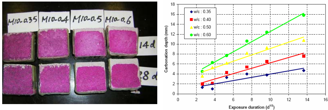
Figure 5A – Carbonation depths measured with phenolphthalein on various mortar samples exposed to a 50% RH 5% CO 2 environment. 5B – Carbonation depths plotted against the square root of time. (Data provided by the author)
