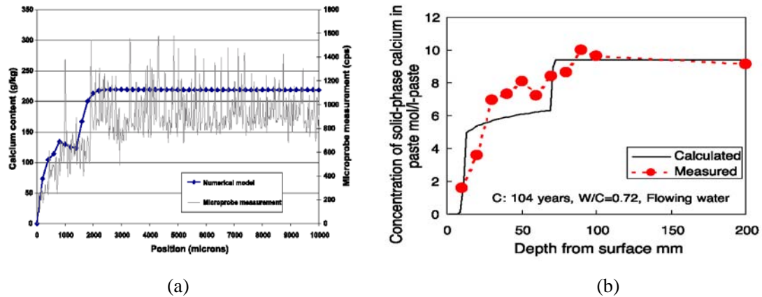
Figure 11 – Simulations of calcium leaching: (a) on cement paste [Maltais04] and (b) on mortar [Yokozeki04]
