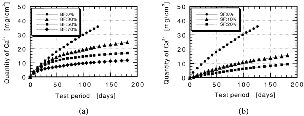
Figure 8 – Cumulative quantity of dissolved \text{Ca}^{2+} for SCM mixtures: (a) blast-furnace slag (BF) and (b) silica fume (SF) [Saito00]
