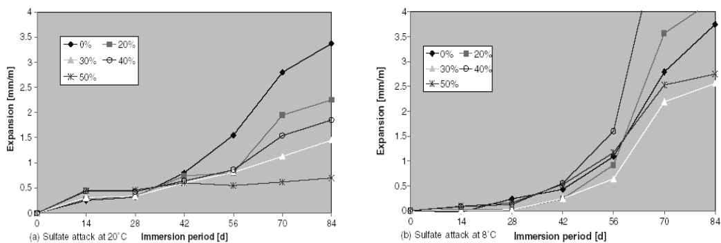
Figure 15 – Expansions of PLC mortar prisms containing fly ash after immersion in 4.4 % sodium sulfate solution [Mulenga2003]
