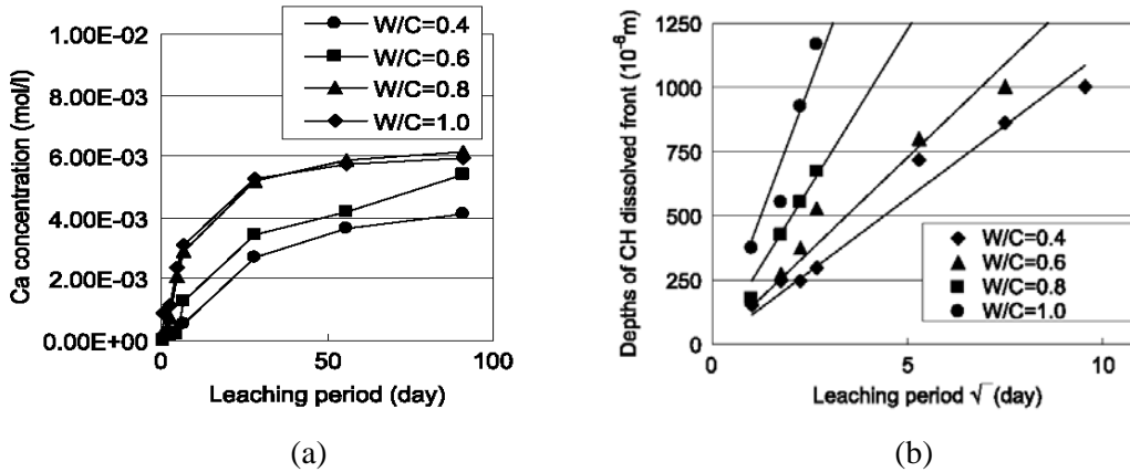
Figure 6 – Change of \text{Ca}^{2+} concentration with the leaching period (a) and depth of the \text{Ca}(\text{OH})_2 dissolved front as a function of the square root of the leaching period (b) [Haga05]
