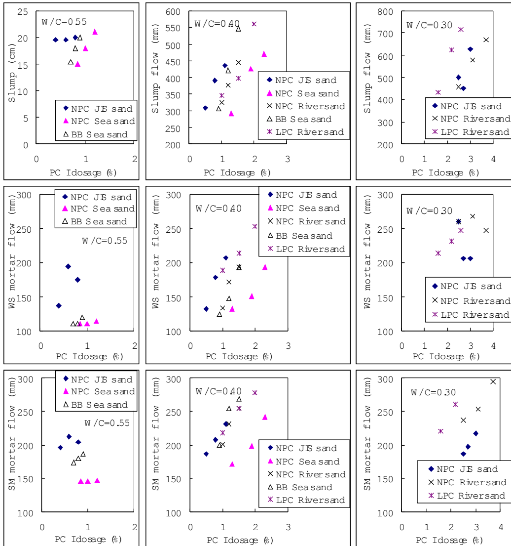
Fig. 17 Relationship between fluidity (concrete slump, wet screened mortar flow, and separately mixed mortar flow) and PC dosage at various W/C [39]. (NPC: Ordinary Portland cement, BB: 50% Blastfurnace slag cement, LPC: Low heat Portland cement)
