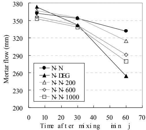
Fig. 32 The effect of DEG addition on the fluidity of mortar containing PC [51].
