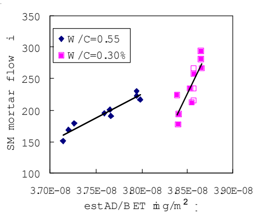
Fig. 19 Estimated adsorption amount of PC per surface area of hydrated cement and flow of separately mixed mortar [39].
