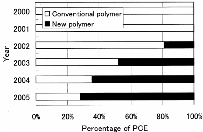
Fig. 6 Consumption volume percentage of total PC-based superplasticizers in Japan [11].
