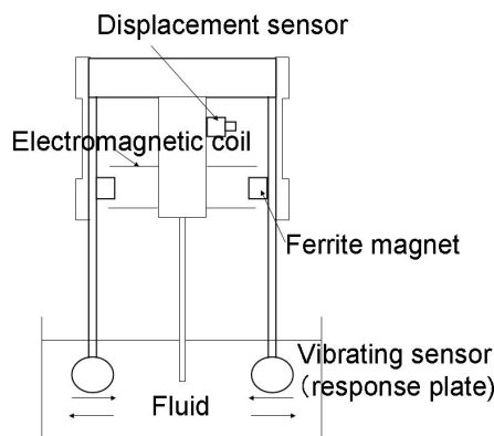
Fig.3 Schematic diagram of vibrating viscometer.
