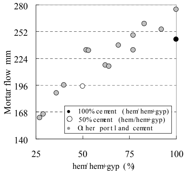
Fig. 29 The effect of hemihydrate ratio on the fluidity of mortar containing PC [47].
