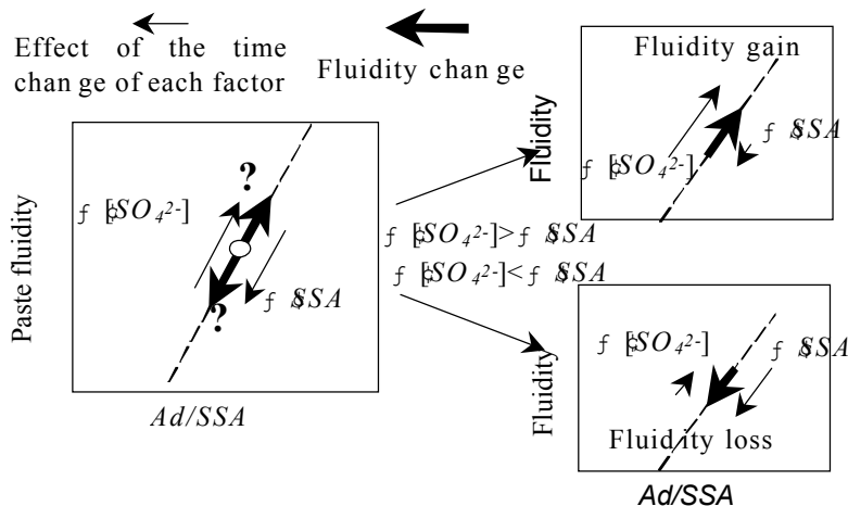
Fig. 13 Fundamental concept of the working mechanism of the time change of paste fluidity containing PC [23].
