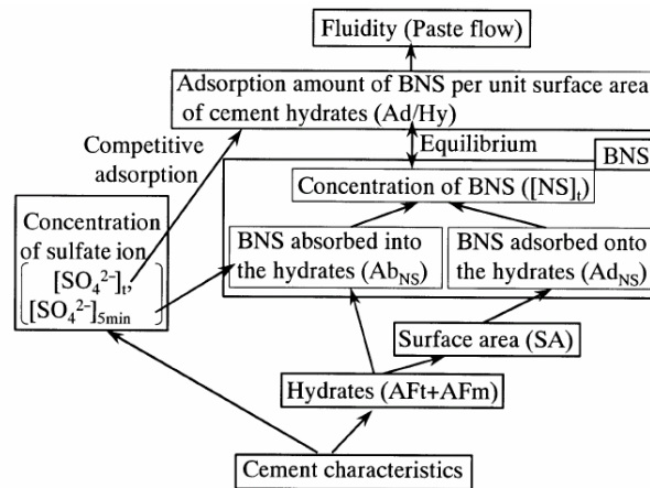
Fig. 15 Modeling the working mechanism of PNS [38].
